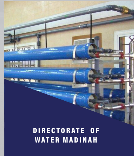
Reverse Osmosis Plant At Wadi Al Fara
